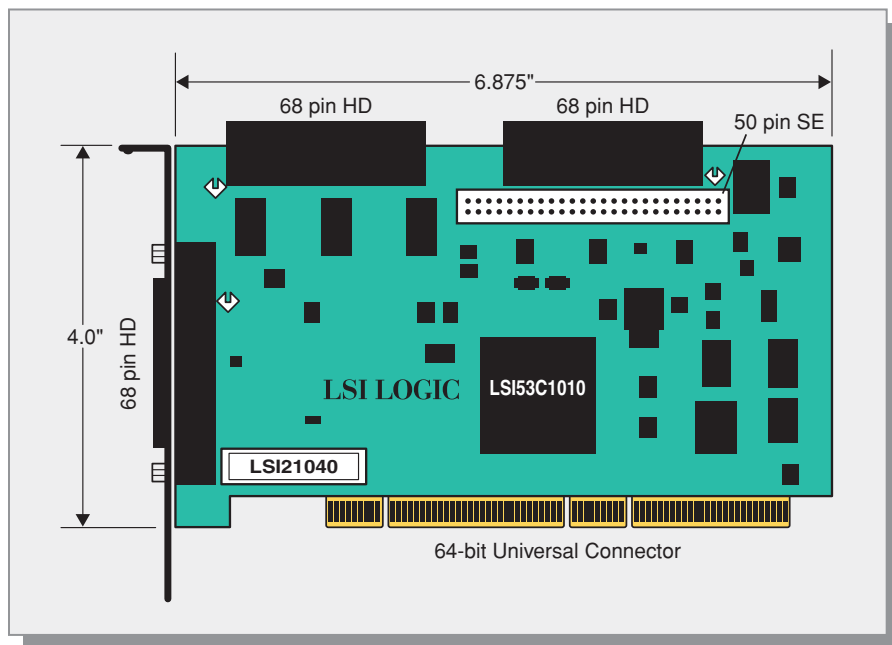
Figure 1: LSI21040 host adapter
