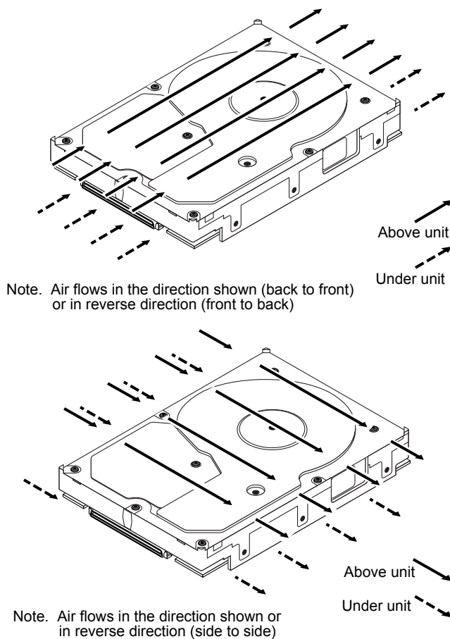
Figure 21. Air flow (suggested)
