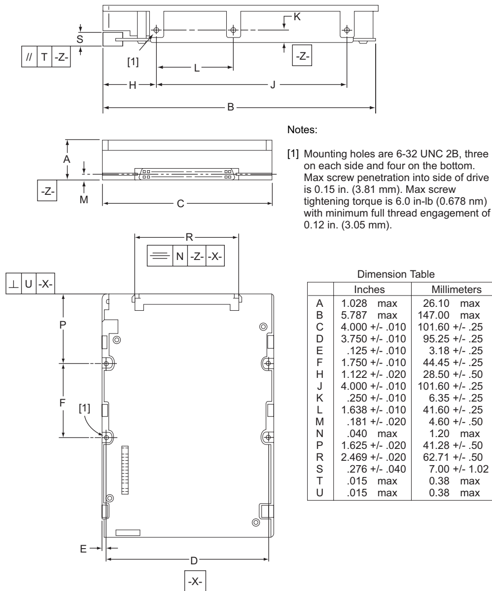
Figure 17. LC mounting configuration dimensions
