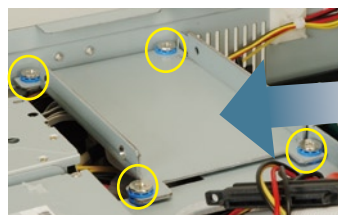
Shock Test
