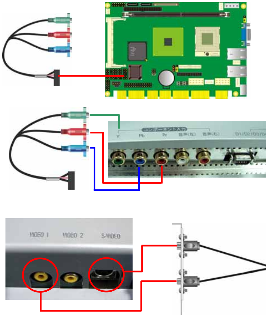
YPrPb Component Cable (For HDTV)
