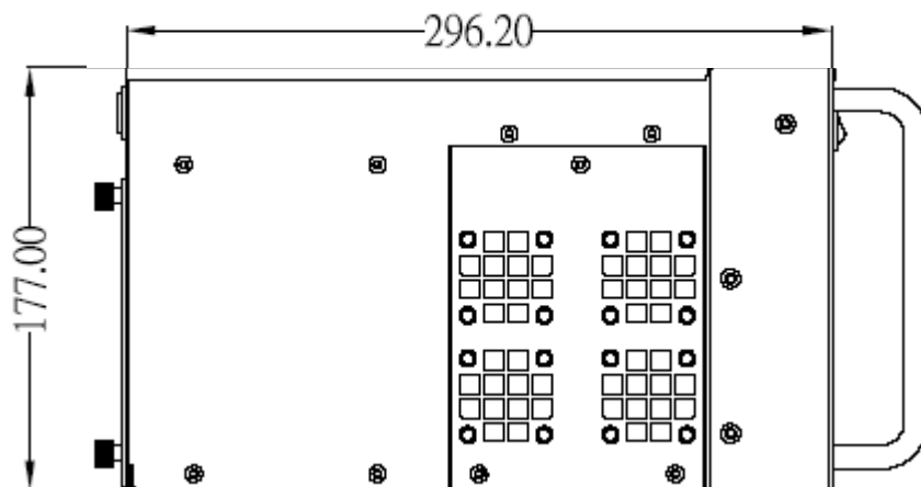
Figure 1-6: cPCIS-6400 Series Left Side View
