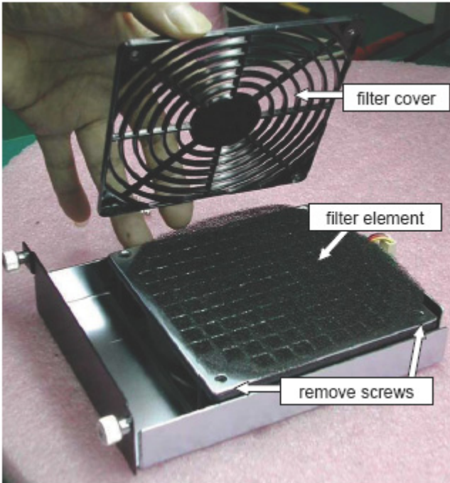
Figure 4-9: Air filter removal and replacement
