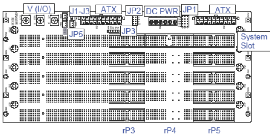
Figure 3-4: cBP-6405R Backplane Rear View
