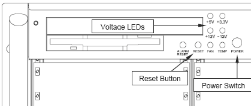
Figure 2-7: cPCIS-6400U Series switches and LEDs
