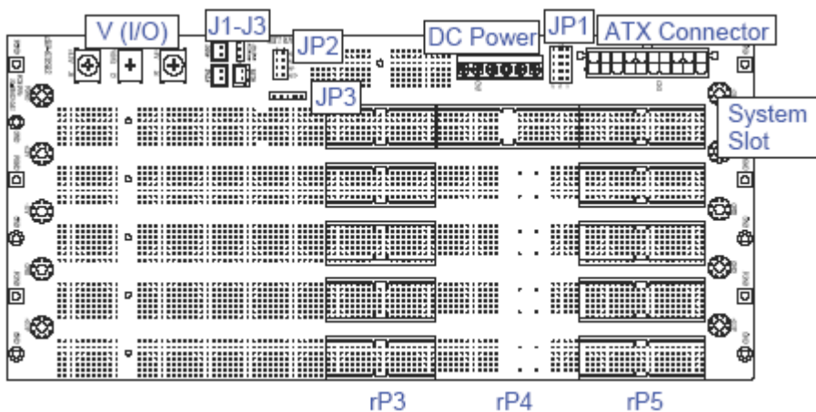
Figure 3-2: cBP-6105R Backplane Rear View
