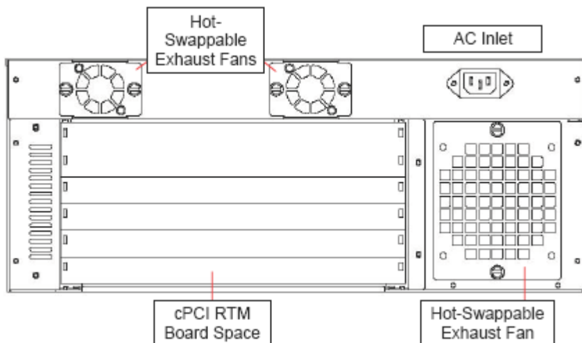
Figure 1-2: cPCIS-6400U Rear View
