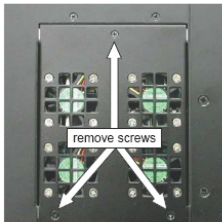
Figure 4-7: Remove the left-side exhaust fan module screws
