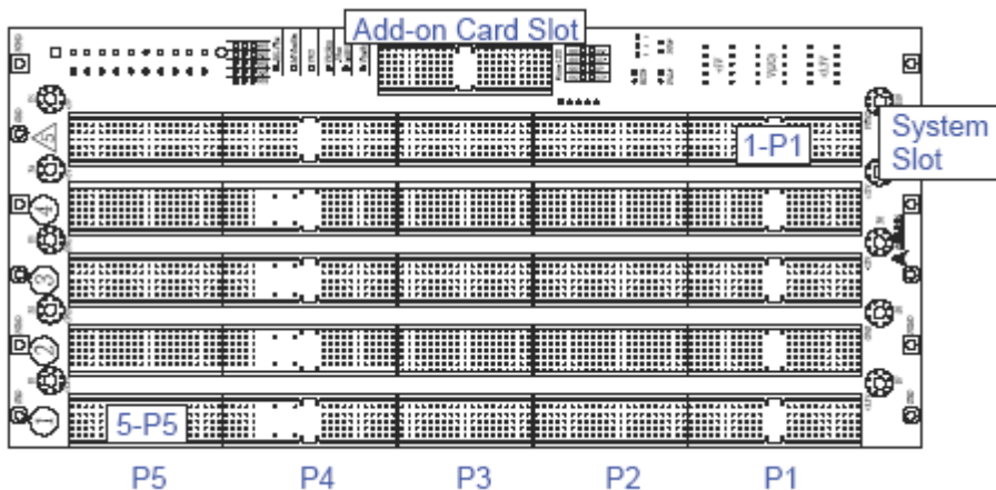
Figure 3-3: cBP-6405R Backplane Front View
