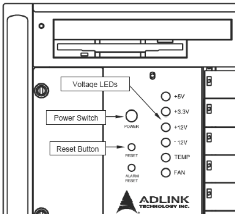
Figure 2-8: cPCIS-6400X Series switches and LEDs
