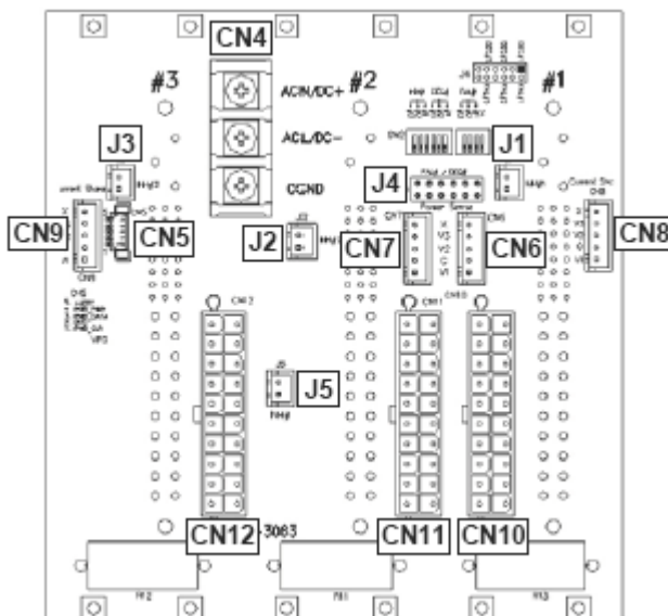
Figure 3-6: cBP-3063 Power Backplane Rear View
