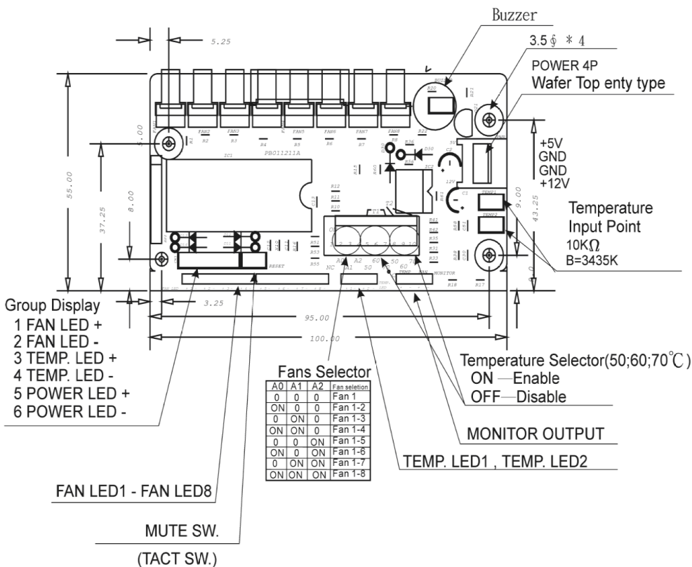
Figure 4-1: System Alarm Board Mechanical Drawing
