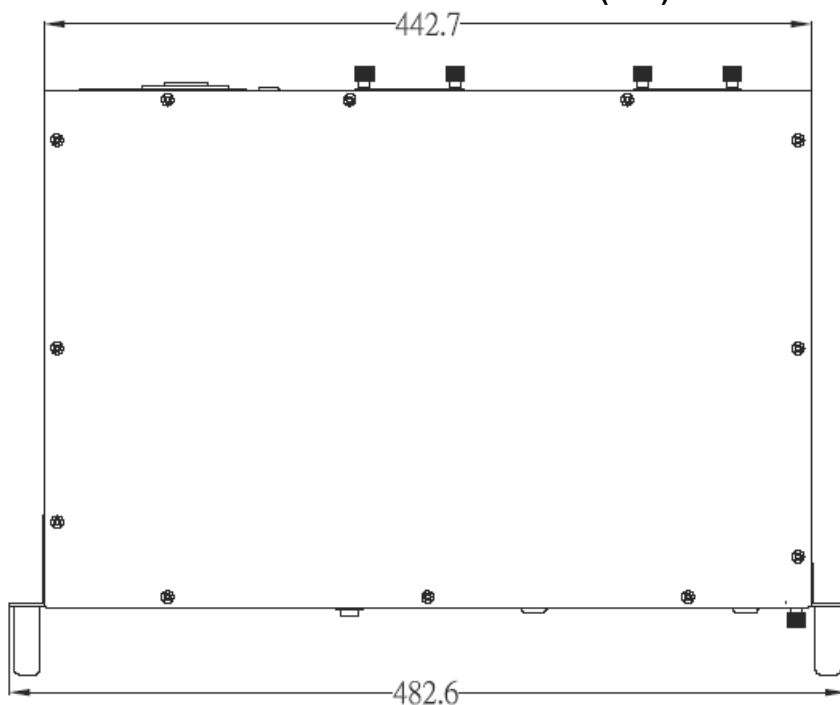
Figure 1-5: cPCIS-6400 Series Top View
