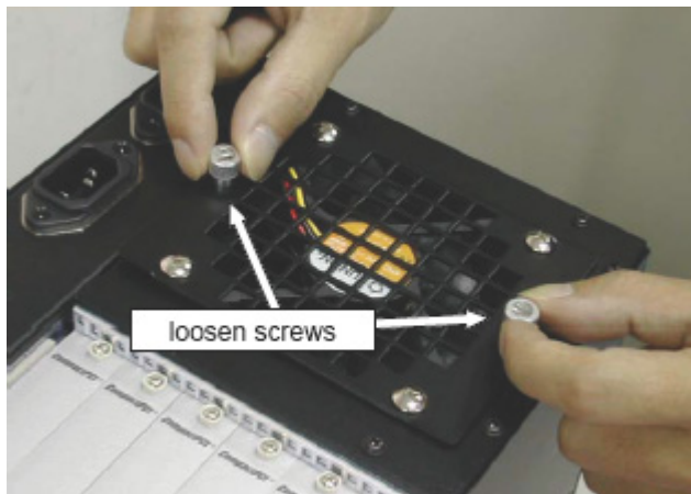
Figure 4-5: Remove the rear exhaust fan module (PSU)
