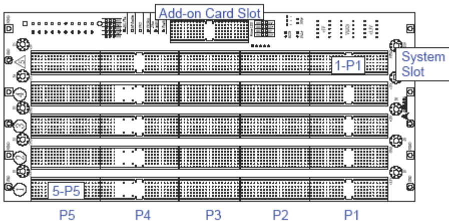
Figure 3-1: cBP-6105R Backplane Front View
