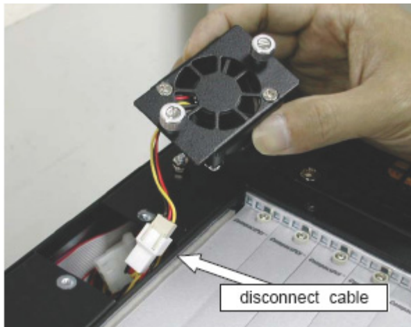
Figure 4-4: Remove the rear exhaust fan module (small)
