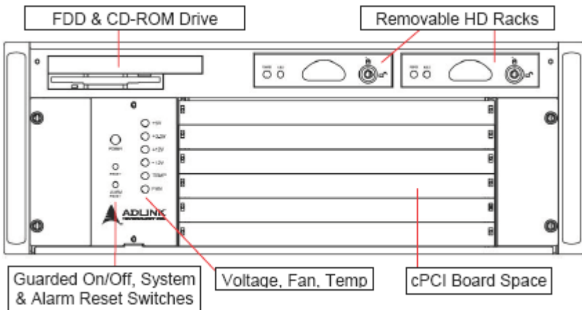
Figure 1-3: cPCIS-6400X Front View
