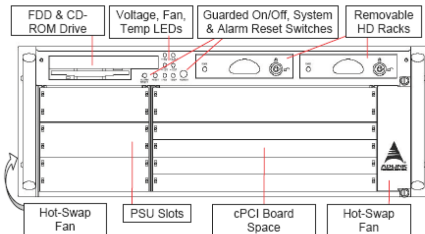
Figure 1-1: cPCIS-6400U Front View
