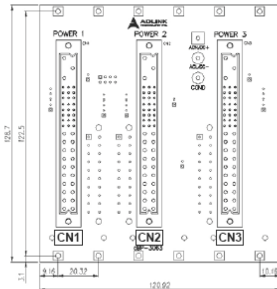
Figure 3-5: cBP-3063 Power Backplane Front View
