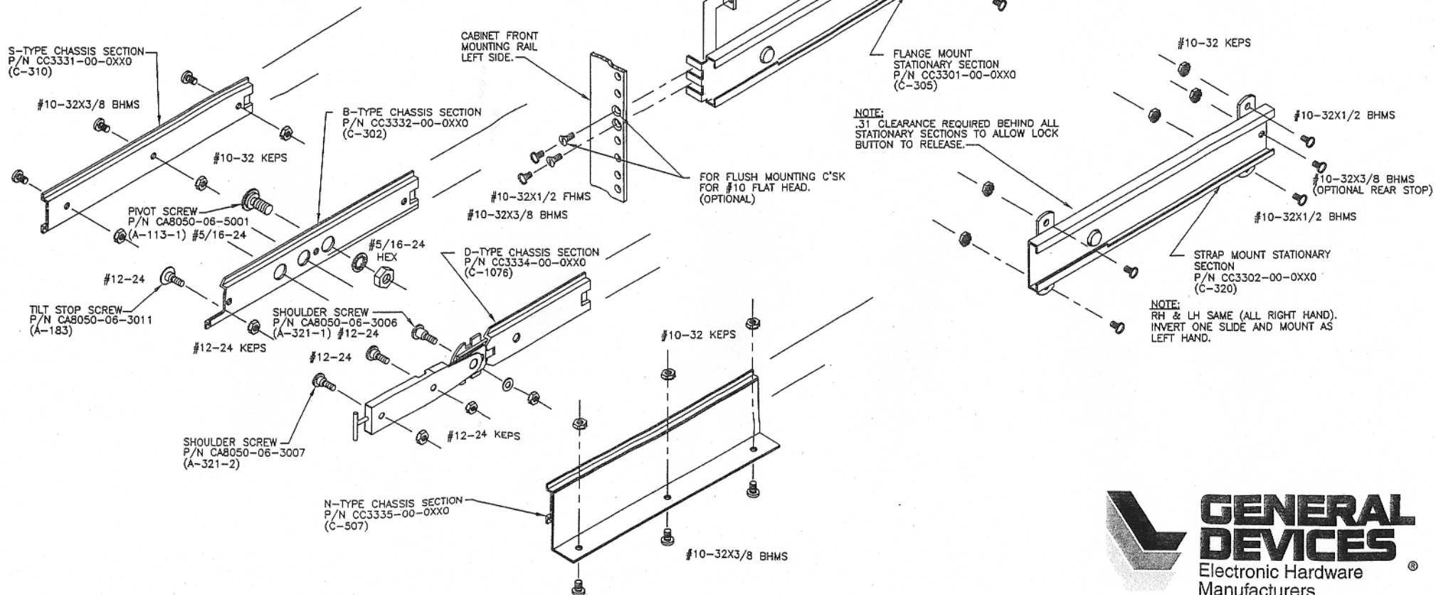
RECOMMENDED MOUNTING
