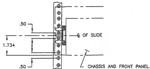
RECOMMENDED MOUNTING
