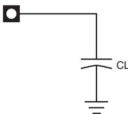
Figure 3. AC Test Loads for General Output Pins
