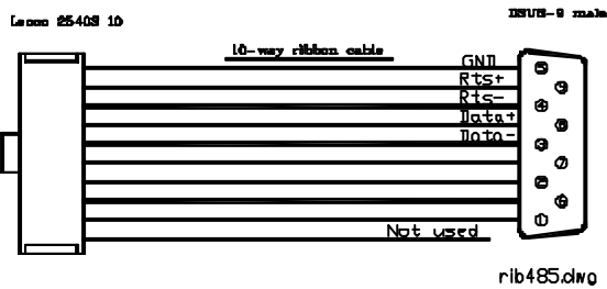
RS/485 CONNECTOR
