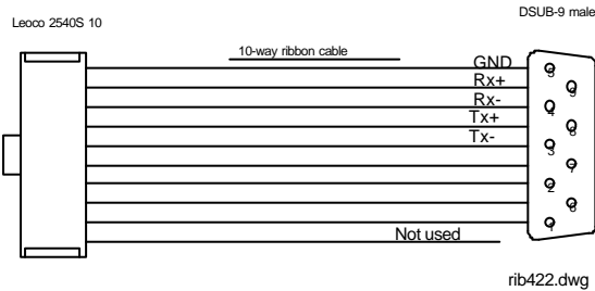
RS/422 CONNECTOR
