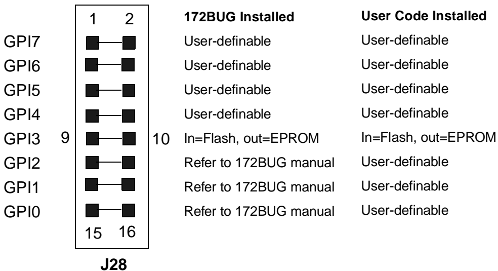
Figure 4-3 MVME172FX Jumper Settings
