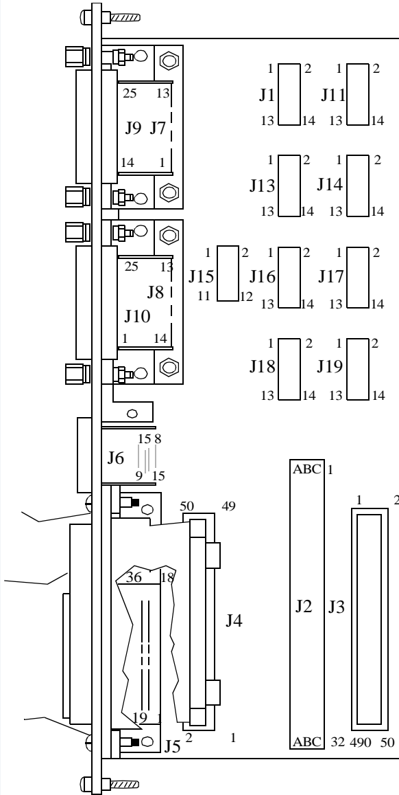
Figure 6-1 MVME712 Jumper Block Locations
