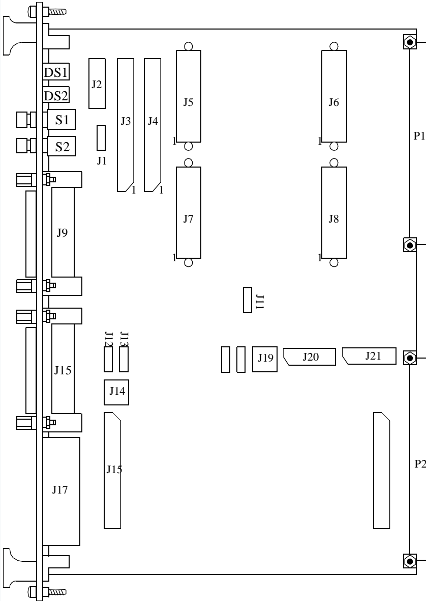
Figure 4-2 MVME172LX Jumper Block Locations
