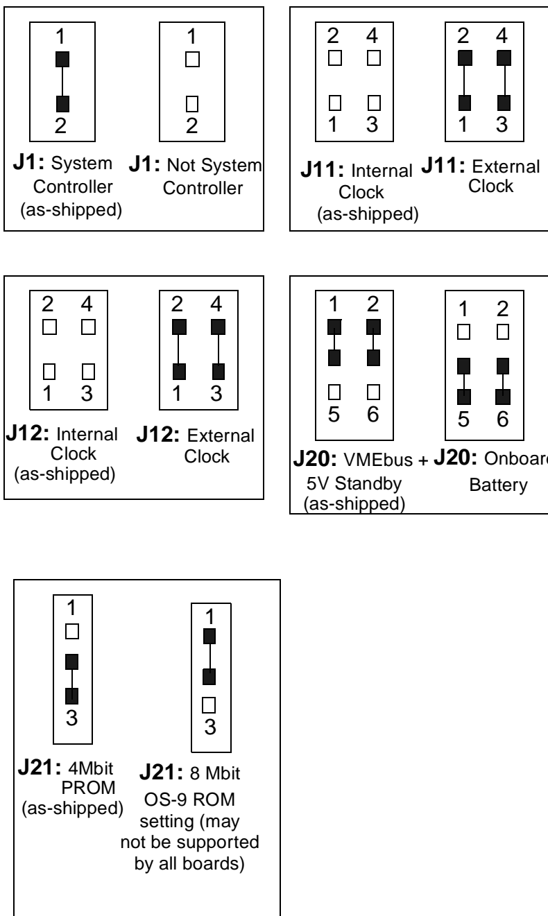
Figure 2-2 Jumper Locations
