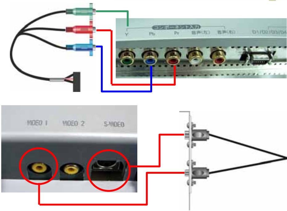
S-Video & Composite Cable (For SDTV)
