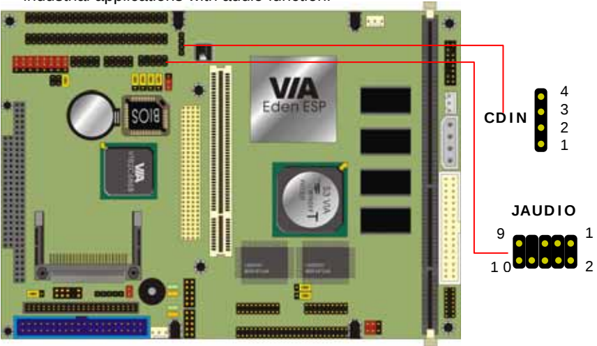
Connector: JAUDIO Type: 10-pin header
